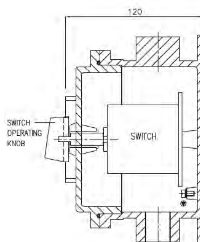
SECTIONAL VIEW
